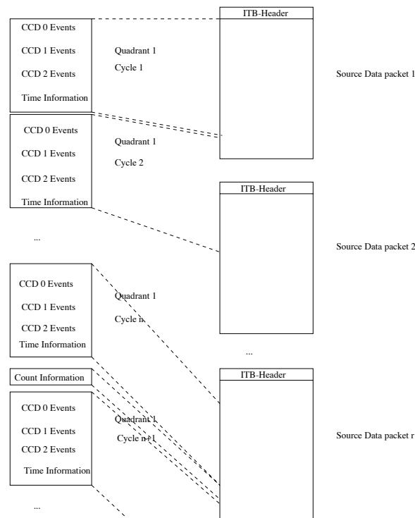
Figure 4: EPIC p-n Full Frame Imaging Mode Data
