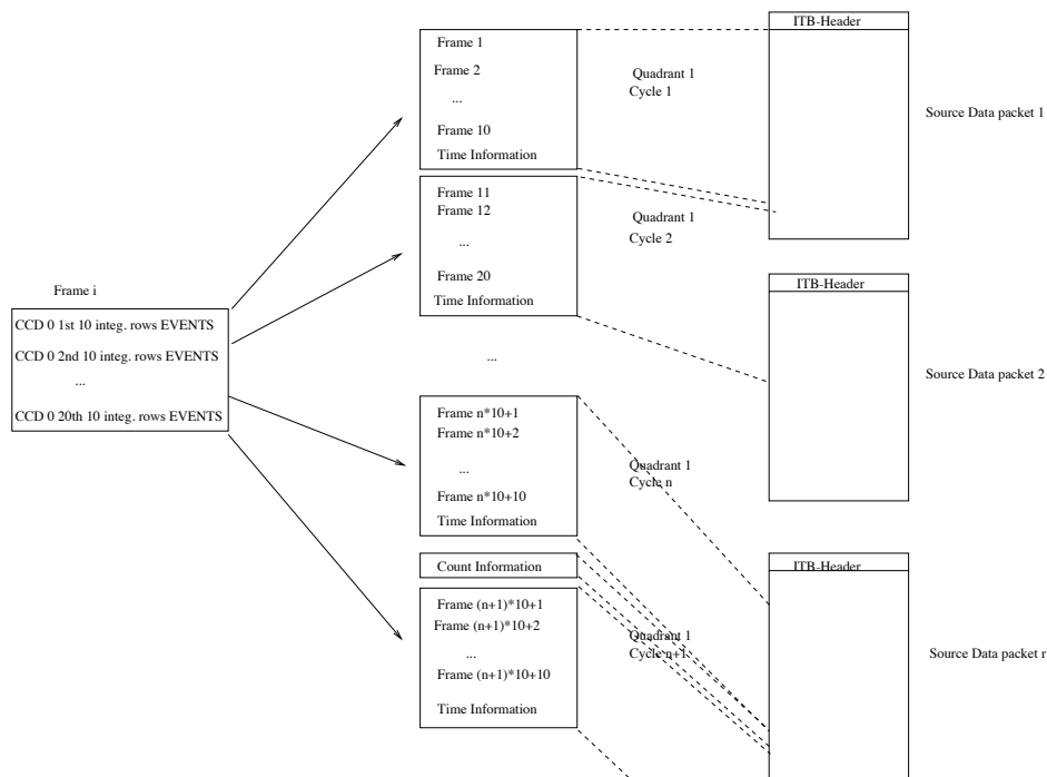
Figure 5: EPIC p-n Timing Mode Data
