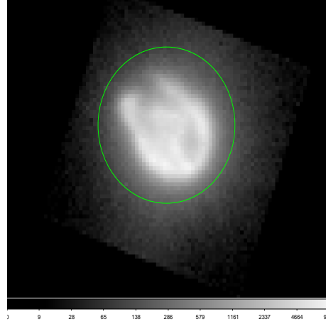
Figure 1: N132D in the EPIC-pn camera, small window. The remnant is enclosed within an 85 arcsecond radius circle.
