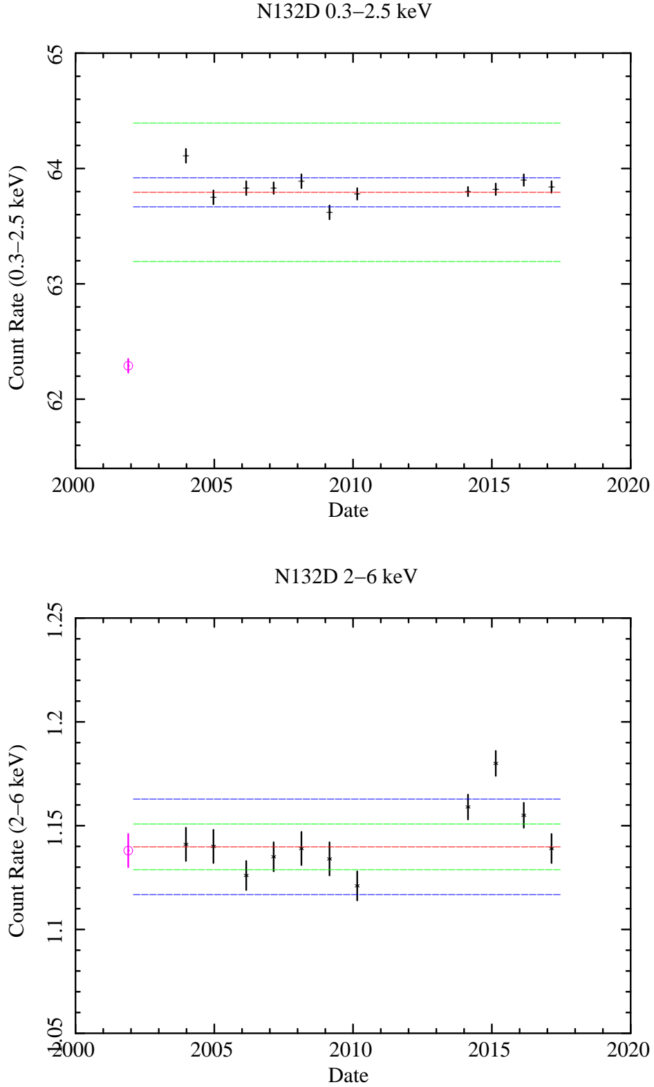
Figure 3: Upper: 0.3–2.5 keV background-subtracted count rate from a circle of radius 85 arcseconds centred on N132D. The dashed red line gives the mean value of 63.8 c/s while the blue and green dashed lines give a variation of 0.2% and 1% about this mean respectively. All observations were made with the thin1 filter except that of 2001-10-20 which was made with the medium filter and is shown in magenta. Lower: 2–6 keV background-subtracted count rate from N132D. The mean rate of 1.4 c/s is shown as a dashed red line while the 1% and 2% variations about the mean are shown as green and blue dashed lines respectively.
